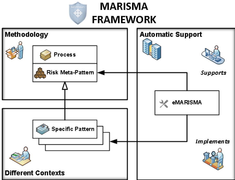
Fig. 3 General architecture of the MARISMA framework
